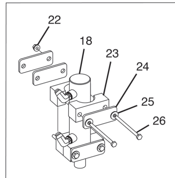
Cylinder configuration for spreaders with a serial number up to 105-101.
