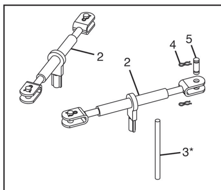
Turnbuckles for Non-steerable Hitch
