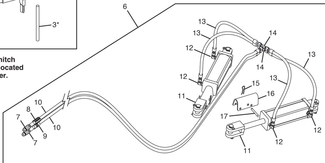
Hydraulic-Driven Steerable Hitch
